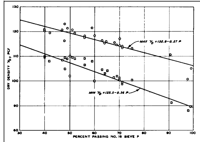
Figure 5-15. Correlation between density and percent passing No. 16 sieve
