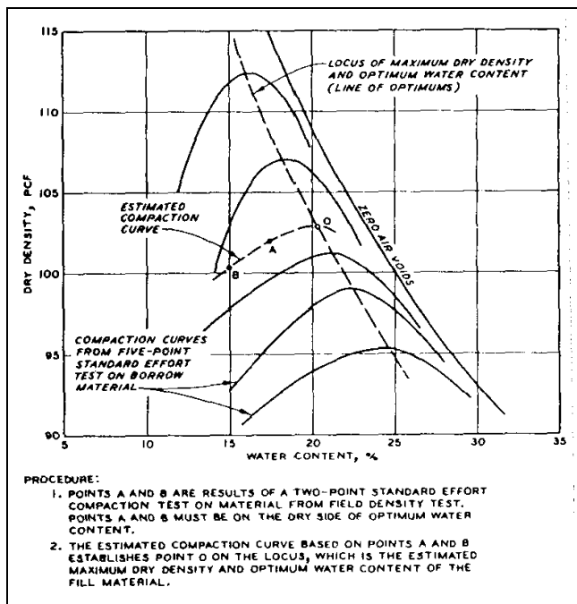
Figure B-3. Illustration of two-point compaction method
