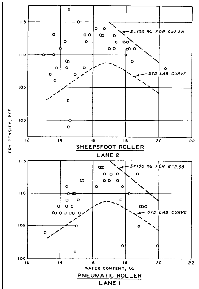
Figure 5-6. Test fill data from Canyon Dam, Texas
