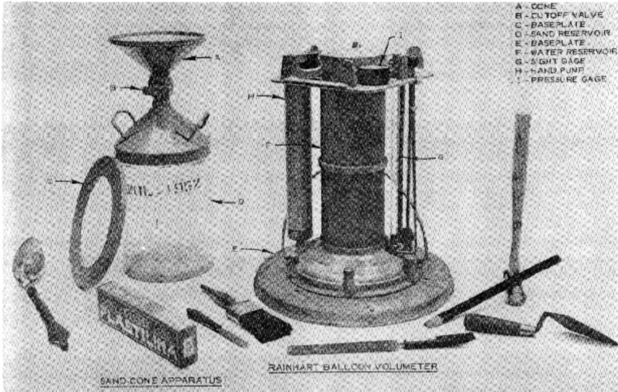
Figure 5-7. Displacement density apparatus
