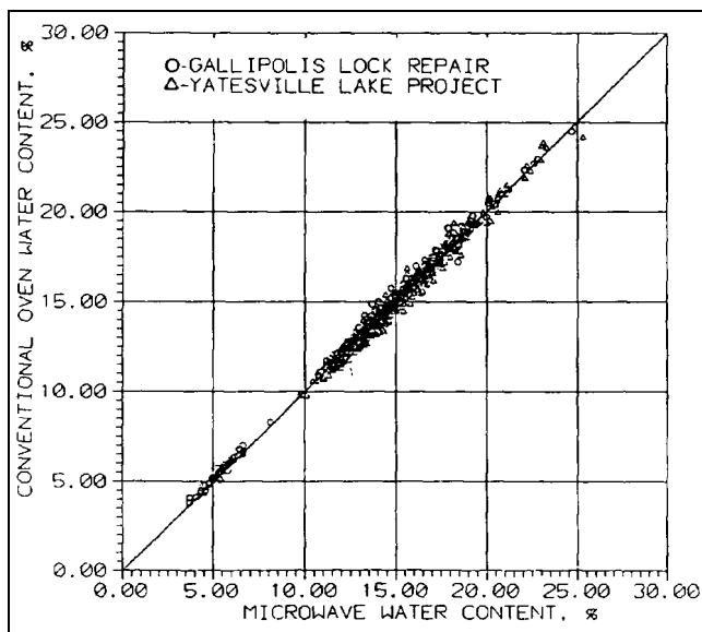
Figure 5-9. Conventional oven versus CCMOS water content data
