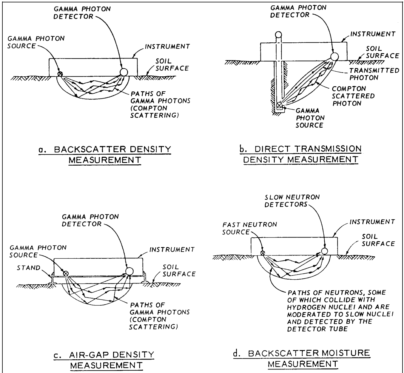
Figure 5-11. Schematic diagrams of density and moisture measurements
