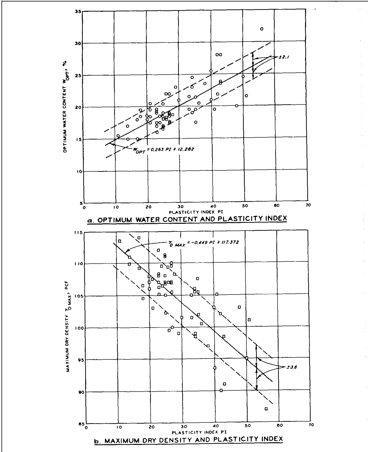
Figure B-5. Examples of plots of optimum water content and maximum dry density versus plasticity index
