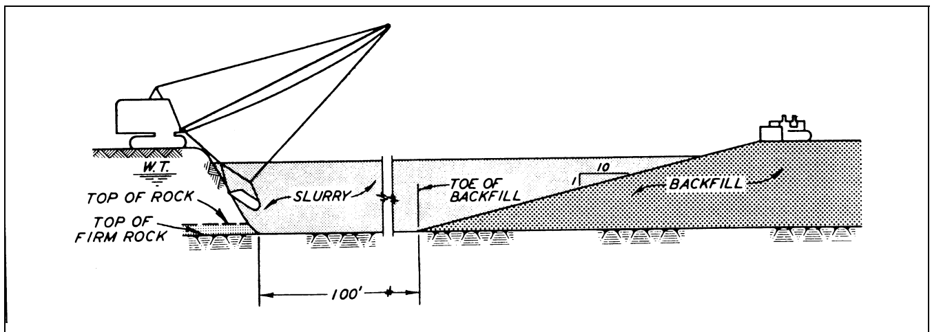
Figure 3-3. Progressive excavation and backfilling scheme for slurry trench construction
