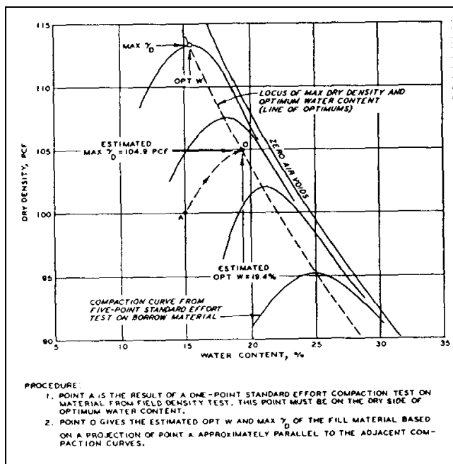
Figure B-1. Illustration of one-point compaction method
